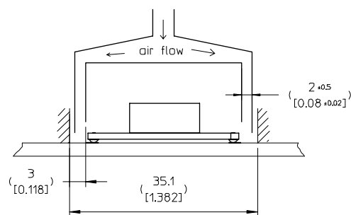
REWORK (REPAIR) (side view)
