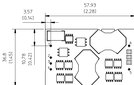
RECOMMENDED FOOTPRINT
