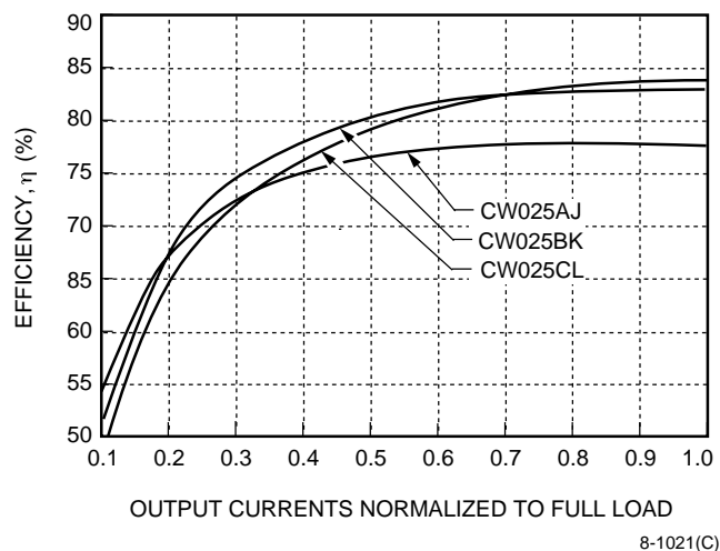
Figure 3. CW025 Dual Output-Series Efficiency vs. Normalized Output Currents (Equal Load on Both Outputs) at V_i = 48\text{ V} and T_c = 25^\circ\text{C}
