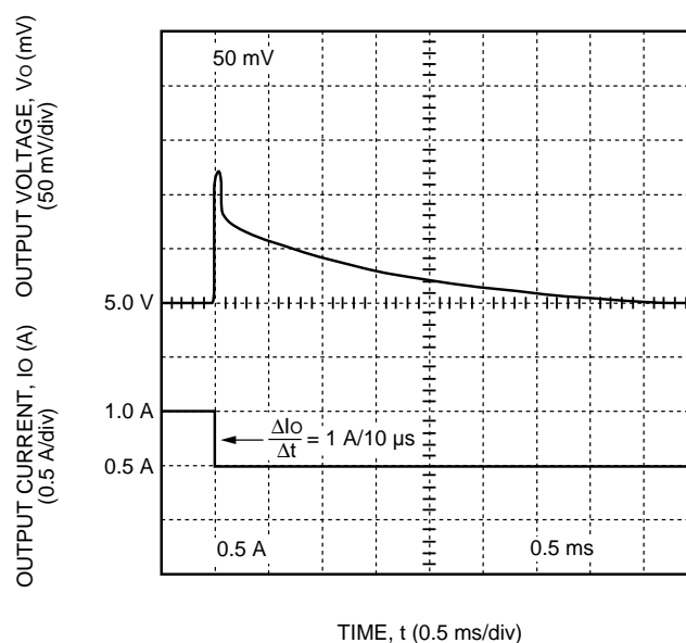
Figure 4. CW025 Dual Output-Series Typical 5 V Output Voltage Response to a Step Load Change from 50% to 25% of I_{o, \text{max}} at V_i = V_{i, \text{nom}} and T_c = 25^\circ\text{C}
