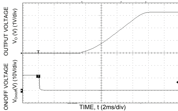
Figure 15. Typical Start-Up Using Remote On/Off with Low-ESR external capacitors ( 7 \times 150 \mu\text{F} Polymer) ( V_{in} = 12.0\text{Vdc} , V_o = 3.3\text{Vdc} , I_o = 3\text{A} , C_o = 1050 \mu\text{F} ).
